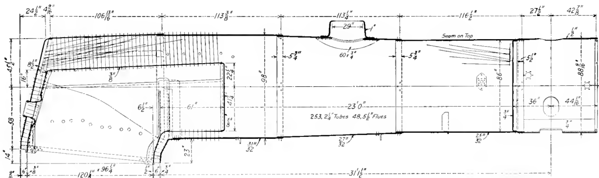
Longitudinal Section of the Boiler for the Wabash 2-10-2 Type Locomotive
